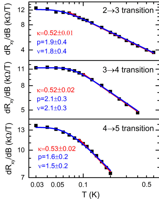
FIG. 2. The slope of Hall resistance at different transitions as a function of temperature (log-log plot). The red lines are fitted by (dR_{xy}/dB)|_{B_c} \propto T^{-\kappa} . The blue lines are fitted by (dR_{xy}/dB)|_{B_c} \propto \tanh(\text{constant} \times T^{-p})^{1/p} , and \kappa is determined by the red fits. The base electron temperature of this measurement system was around 25 \text{ mK} , and the meaningful temperature for the 30 \text{ mK} data points may be higher than the thermometer temperature (lattice temperature). Therefore, the blue fittings start from 40 \text{ mK} .
