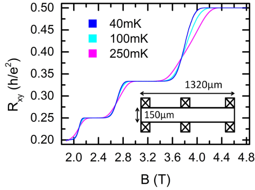
FIG. 1. The Hall resistance as a function of magnetic fields at three different temperatures. The inset shows the size of the Hall bar. Four IQH states are involved in this study: filling factor \nu = 2, 3, 4, 5 . The plateau-plateau transition from filling factor k to k + 1 is labeled as “ k \rightarrow k + 1 ” in this work.
