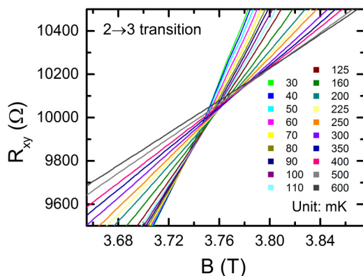
FIG. 3. Zoom-in of the crossing region for the 2 \rightarrow 3 plateau transition.
