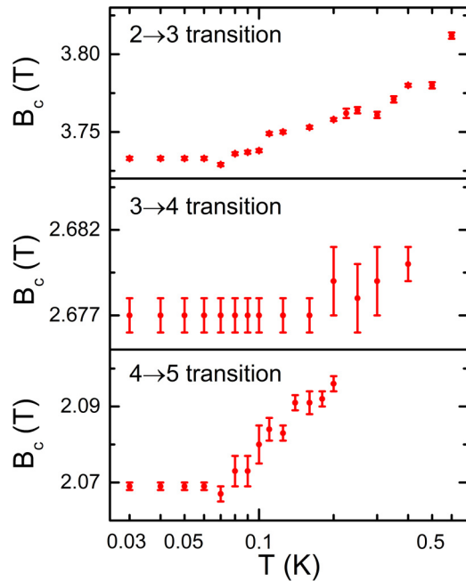
FIG. 5. Temperature dependence of the crossing points at different filling plateau transitions (log-linear plot).
